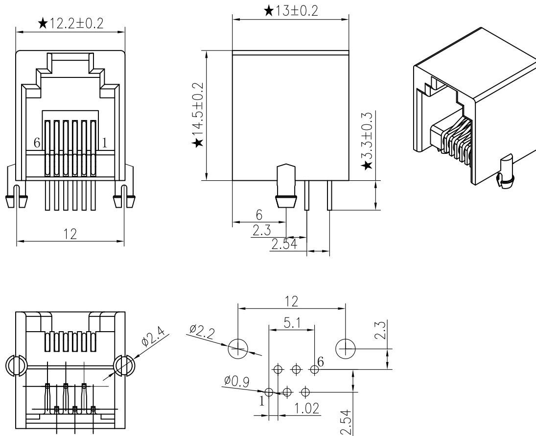
PC BOARD LAYOUT
