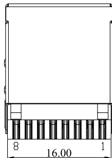
BOTTON VIEW
