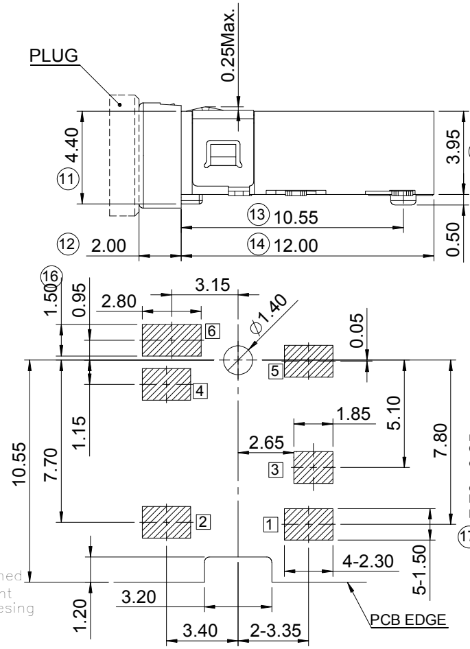
RECOMMENDED PCB LAYOUT(TOP VIEW) (GENERAL TOLERANCE ±0.05)
